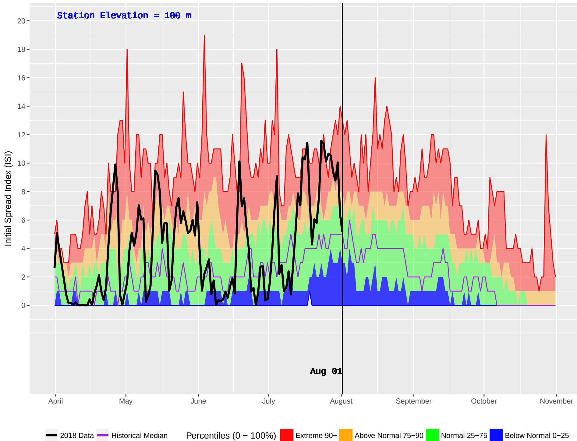
BEAVER CREEK (37) : Historical (1987–2016) and Current (2018) Daily Initial Spread Index (ISI)
